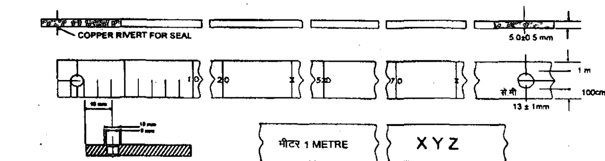
SECTIONAL ENLARGED VIEW OF RIVET
